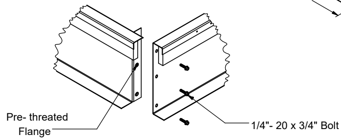
CORNER DETAIL
