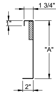
CROSS SECTION DETAIL
