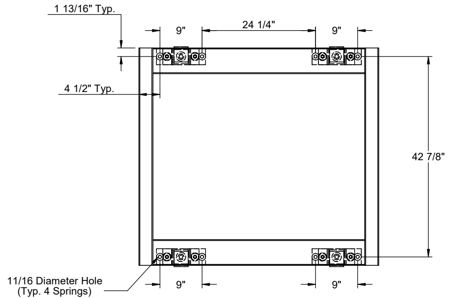
Anchorage Location Detail
