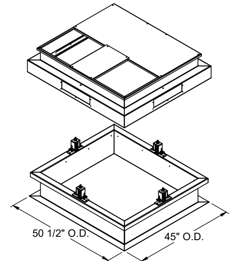
EXPLODED DETAIL
