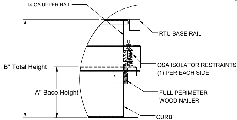
PROFILE DETAIL
