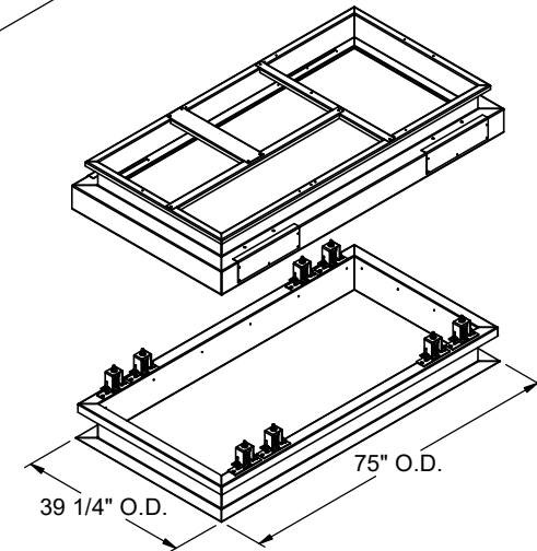
EXPLODED DETAIL
