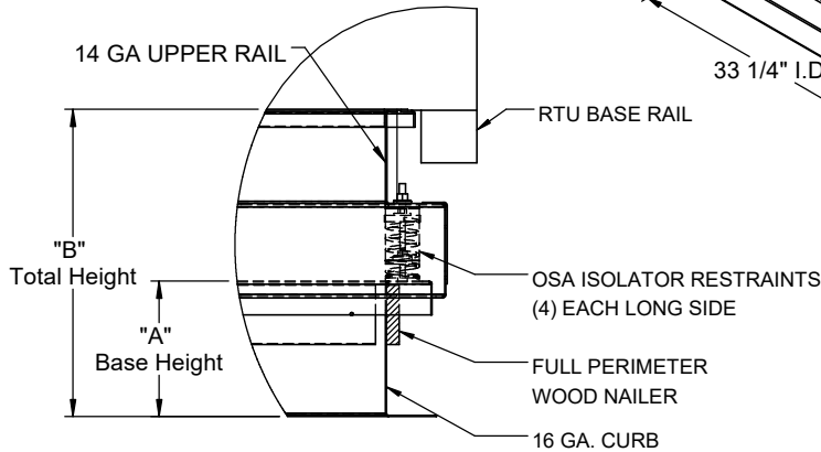
PROFILE DETAIL
