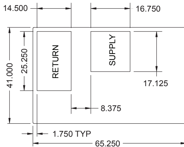
EXISTING CURB
