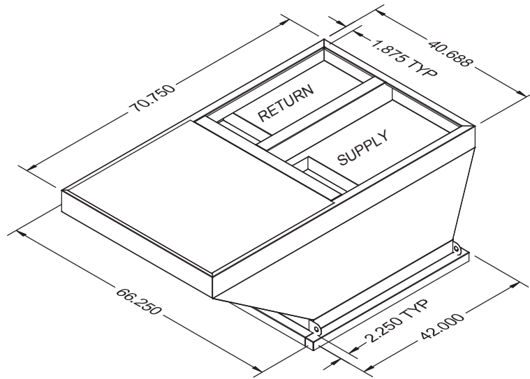
ISO VIEW
