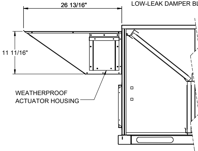
LOW-LEAK DAMPER BLADES
