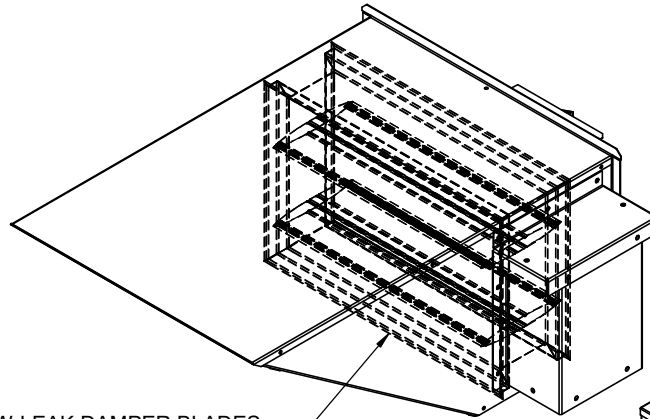
LOW-LEAK DAMPER BLADES
