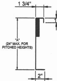
CURB DETAIL
