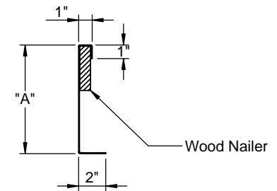
SIDE DETAIL
