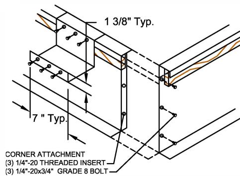
CORNER & HOLD DOWN DETAIL
