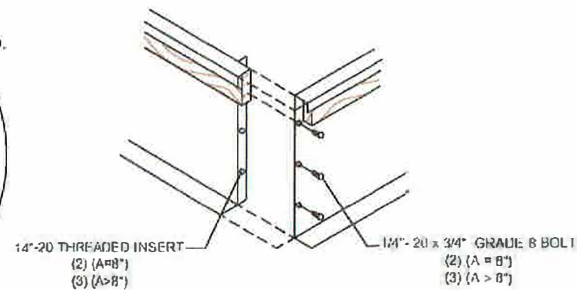
CORNER DETAIL
