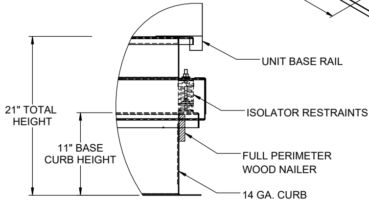
PROFILE DETAIL
