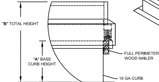
PROFILE DETAIL
