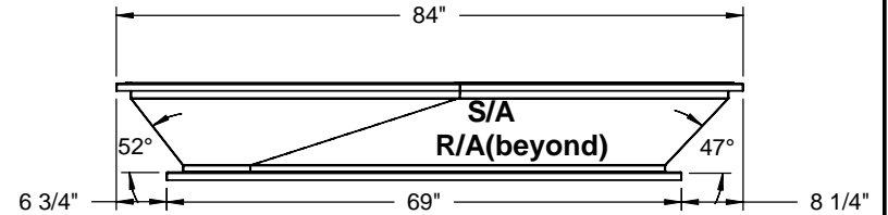
RIGHT VIEW
