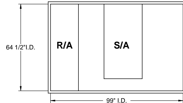
EXISTING CURB
