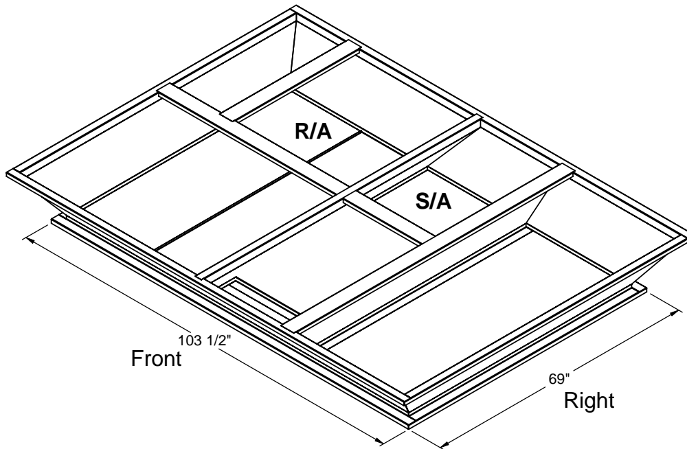
ISOMETRIC VIEW
