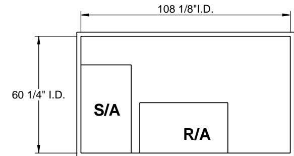
EXISTING CURB
