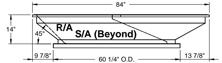
RIGHT VIEW
