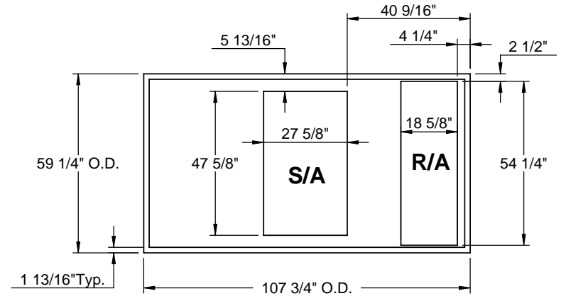
EXISTING CURB
