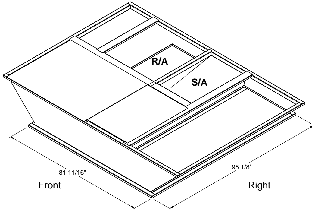
ISOMETRIC VIEW
