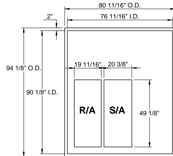
EXISTING CURB
