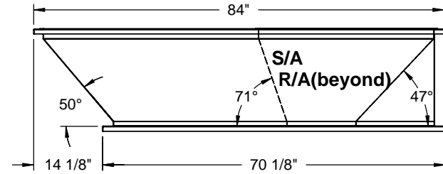
RIGHT VIEW
