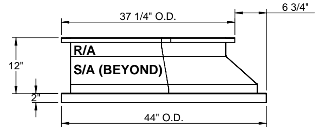
RIGHT VIEW
