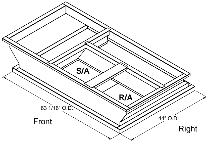
ISOMETRIC VIEW
