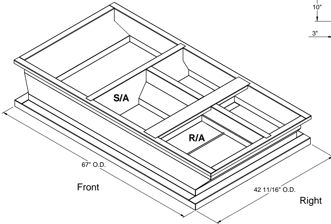
ISOMETRIC VIEW
