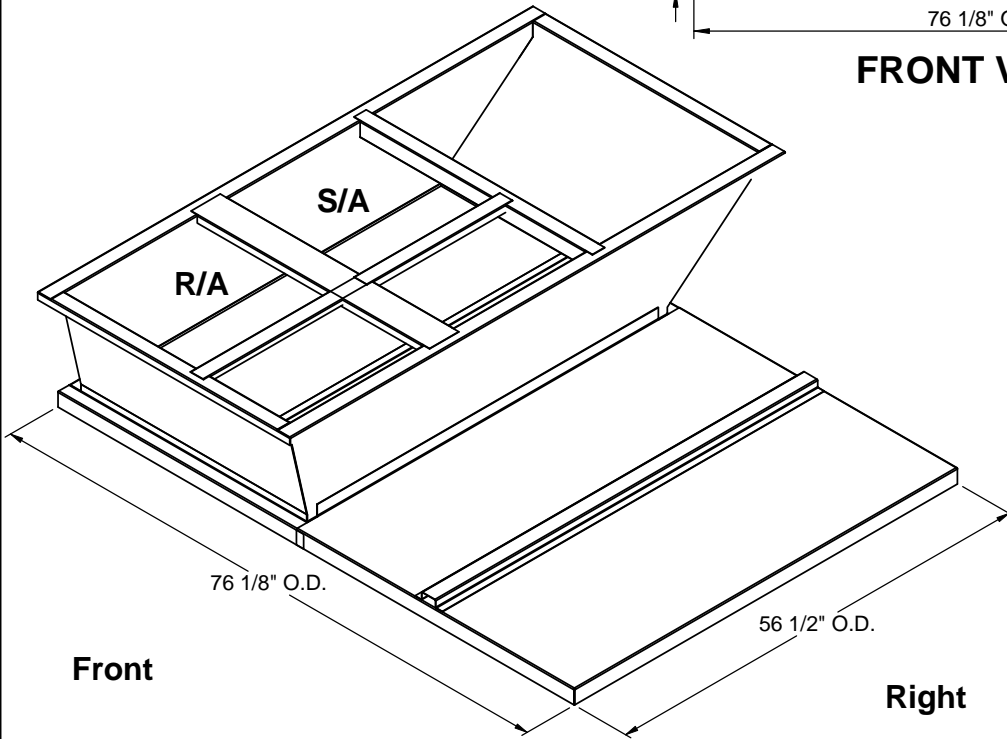
ISOMETRIC VIEW
