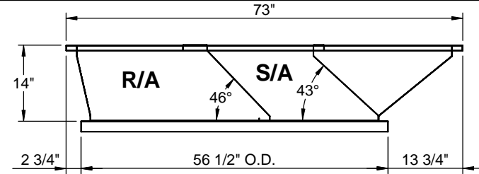
RIGHT VIEW
