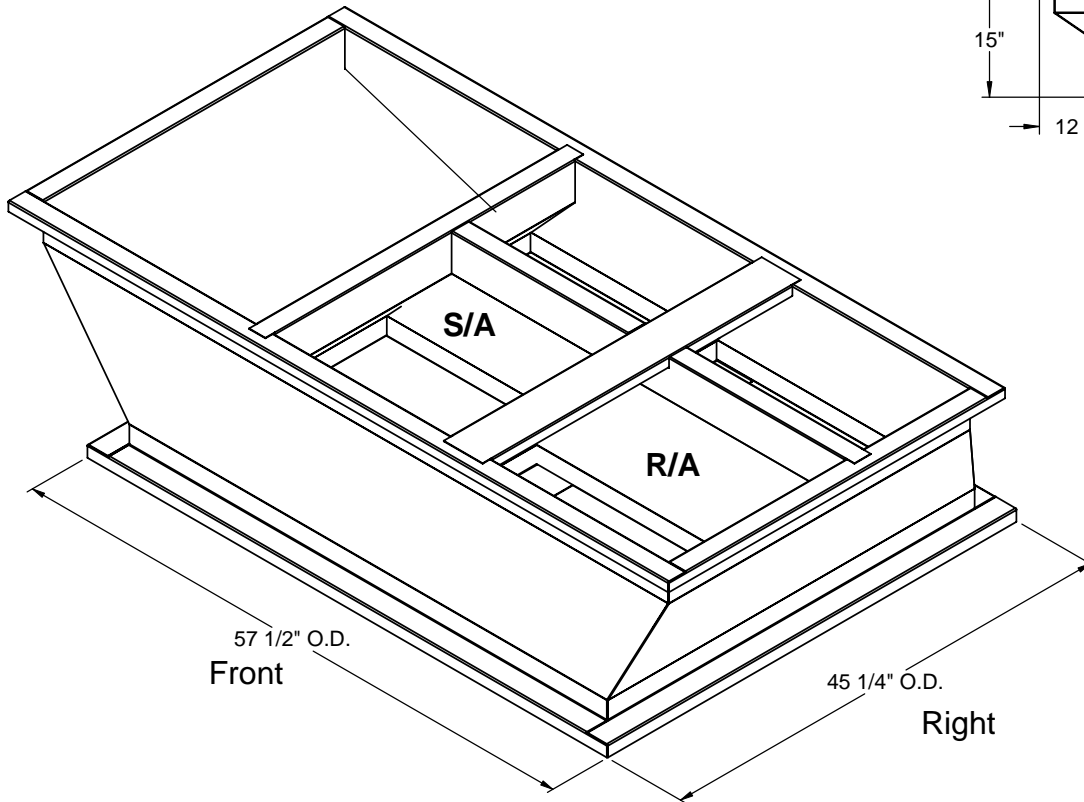
ISOMETRIC VIEW
