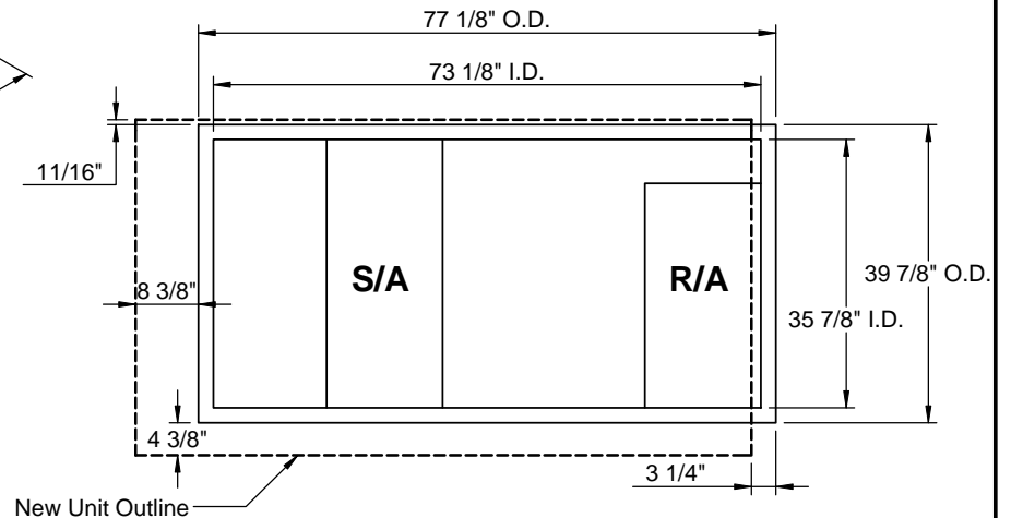
EXISTING CURB
