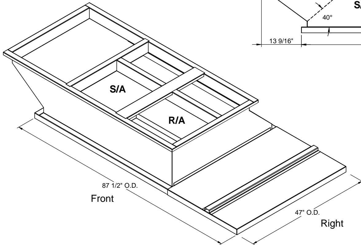
ISOMETRIC VIEW
