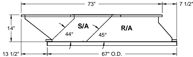
RIGHT VIEW
