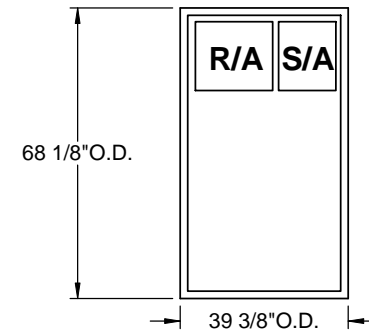
EXISTING CURB
