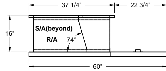
RIGHT VIEW
