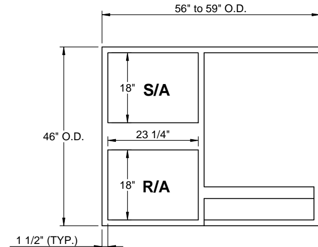
EXISTING CURB
