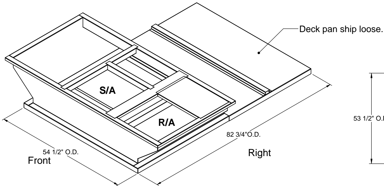
ISOMETRIC VIEW
