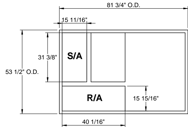
EXISTING CURB
