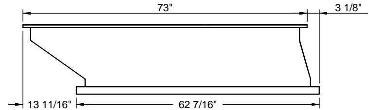
FRONT VIEW
