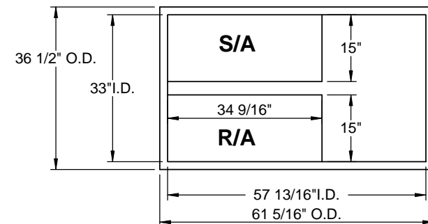
EXISTING CURB
