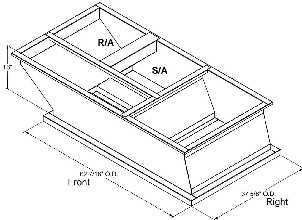
ISOMETRIC VIEW
