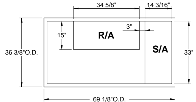
EXISTING CURB
