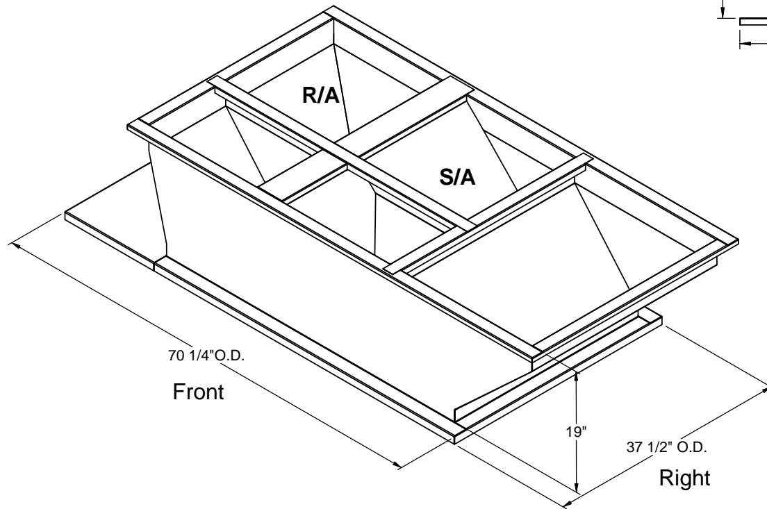
ISOMETRIC VIEW
