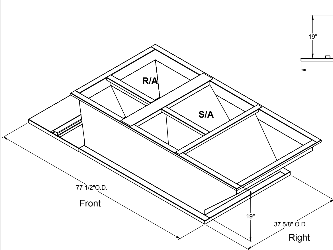
ISOMETRIC VIEW
