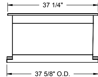
RIGHT VIEW
