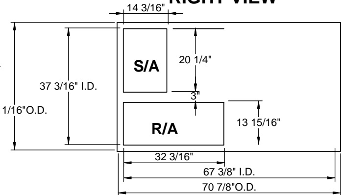
EXISTING CURB
