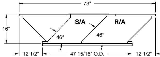
RIGHT VIEW
