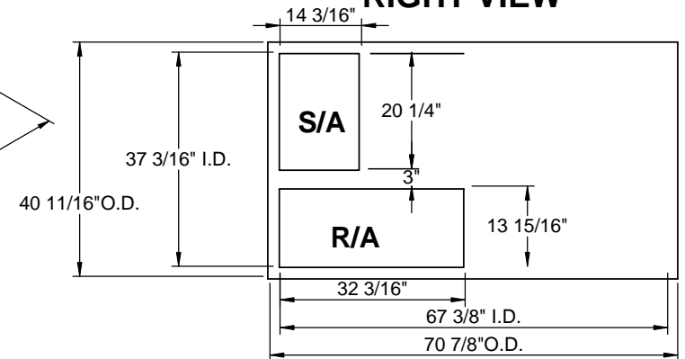
EXISTING CURB
