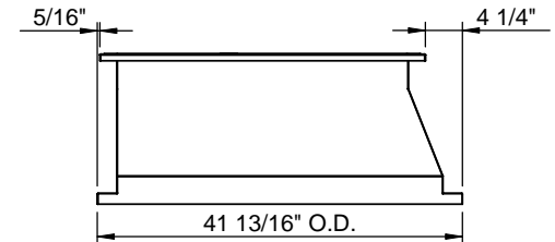
RIGHT VIEW
