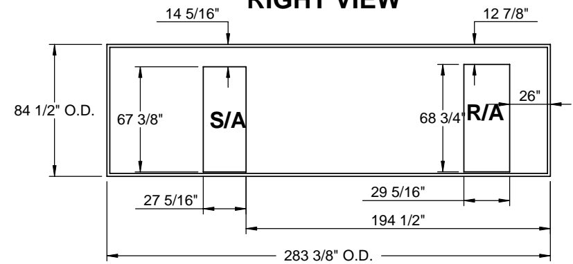
EXISTING CURB
