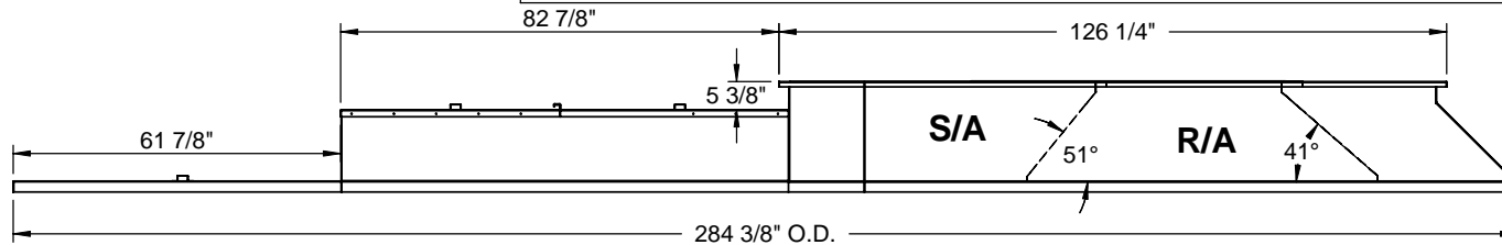
FRONT VIEW
