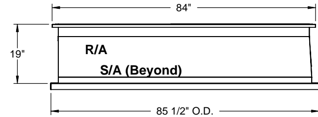
RIGHT VIEW
