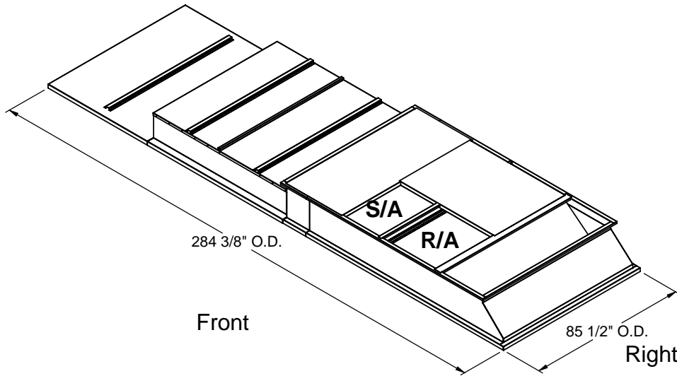
ISOMETRIC VIEW
