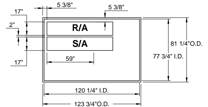
EXISTING CURB
