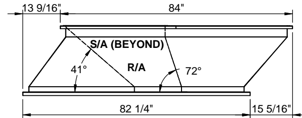
RIGHT VIEW
