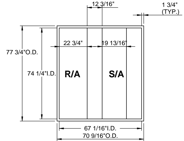
EXISTING CURB
