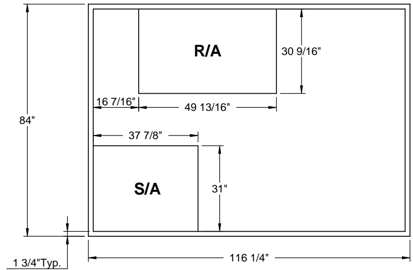
EXISTING CURB
