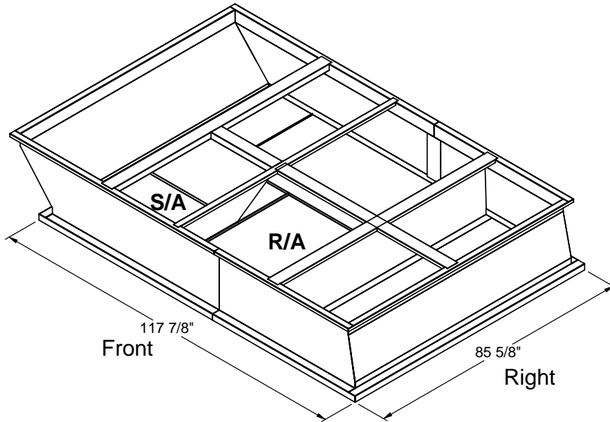
ISOMETRIC VIEW
