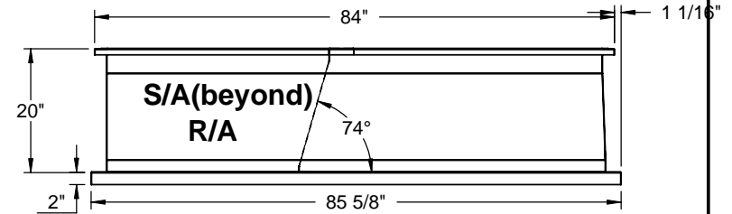
RIGHT VIEW
