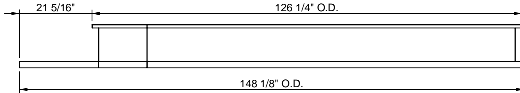
FRONT VIEW
