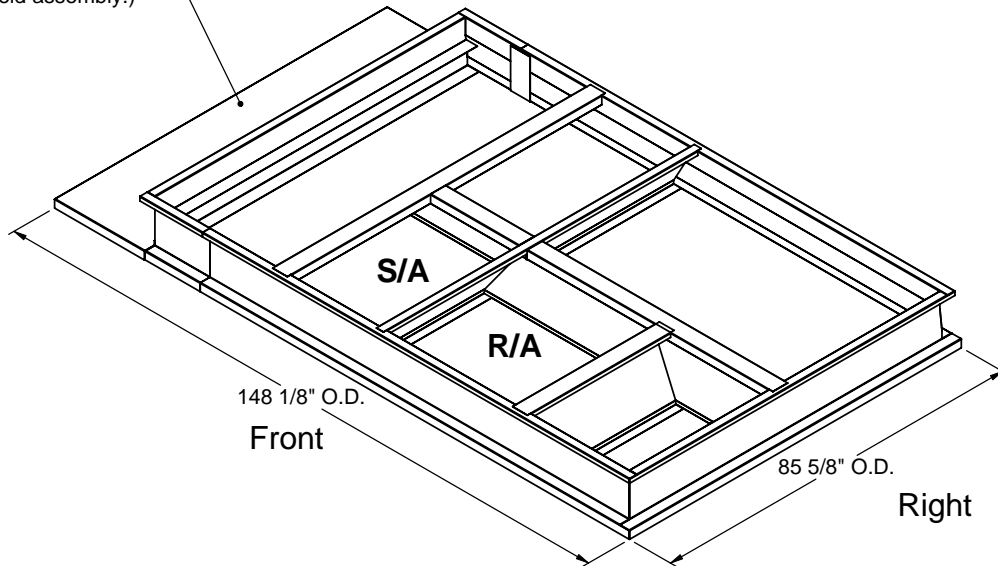
ISOMETRIC VIEW
