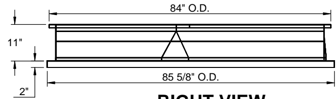
RIGHT VIEW
