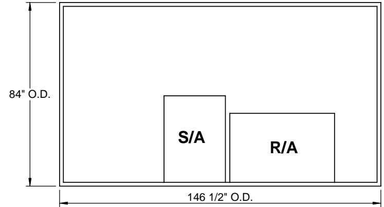
EXISTING CURB
