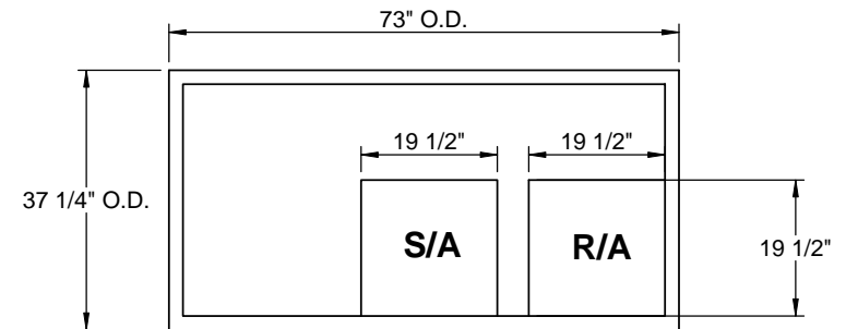
EXISTING CURB
