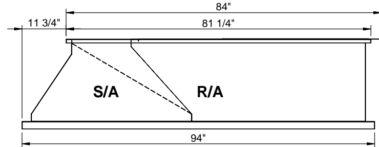
RIGHT VIEW
