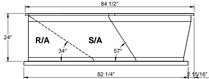
RIGHT VIEW
