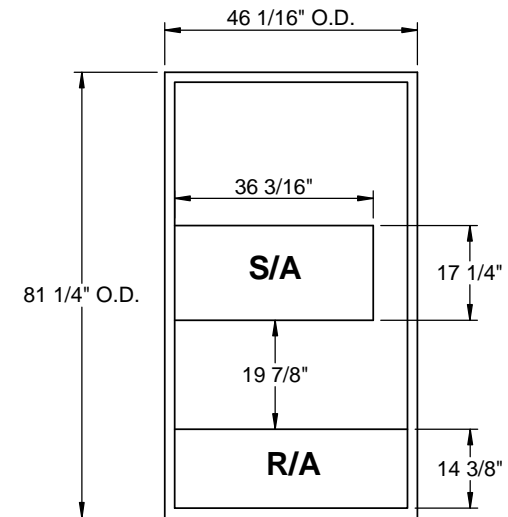
EXISTING CURB
