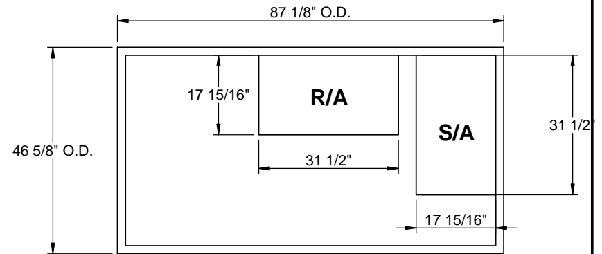
EXISTING CURB
