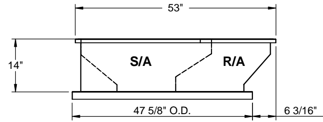
RIGHT VIEW
