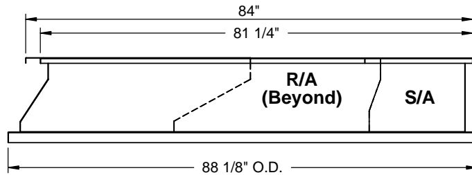
FRONT VIEW
