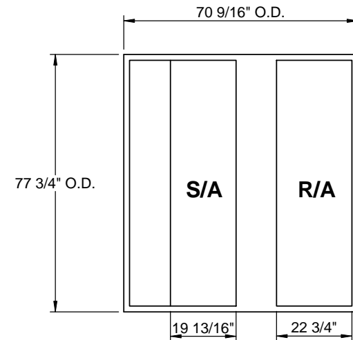
EXISTING CURB
