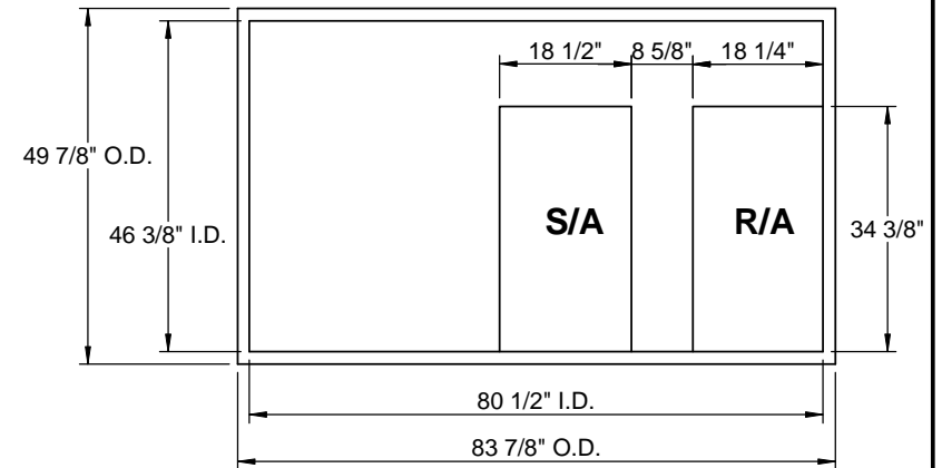
EXISTING CURB
