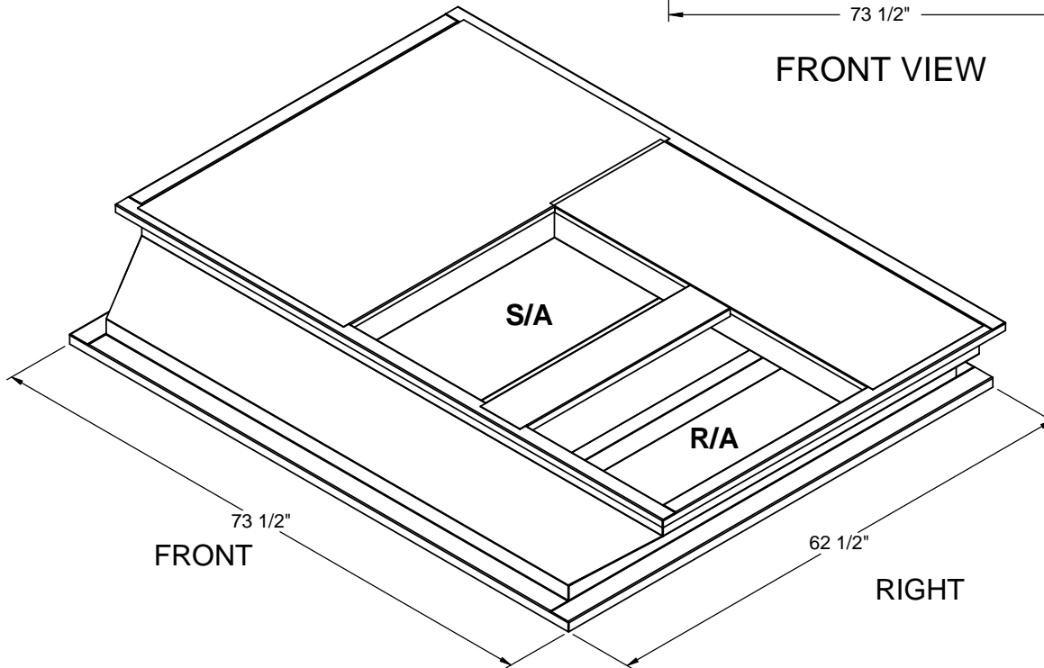
ISOMETRIC VIEW
