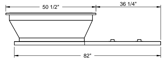
RIGHT VIEW
