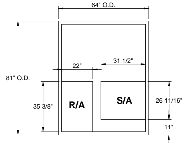
EXISTING CURB
