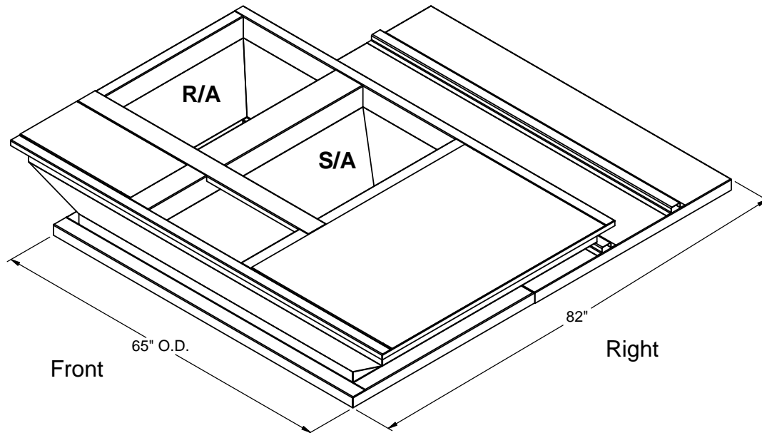
ISOMETRIC VIEW
