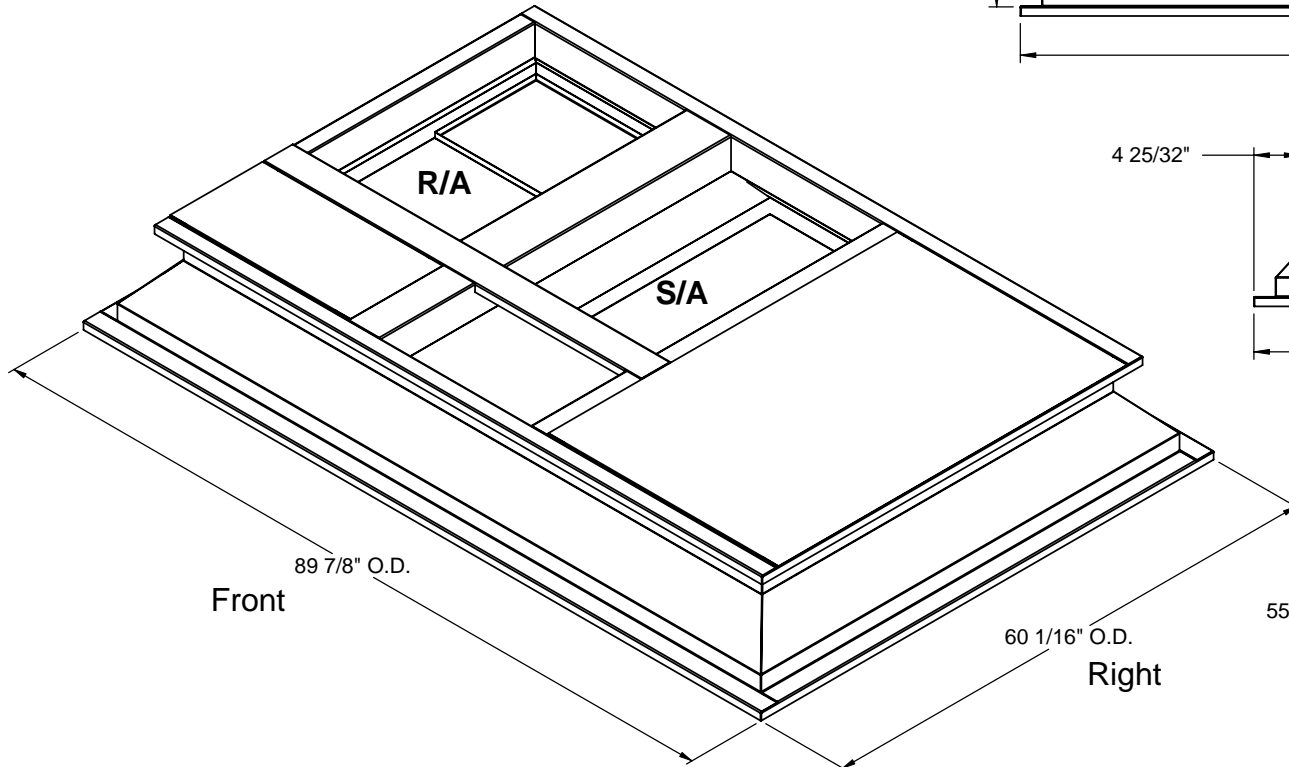
ISOMETRIC VIEW
