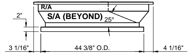
RIGHT VIEW
