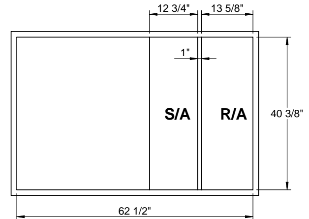
EXISTING CURB
