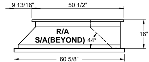
RIGHT VIEW
