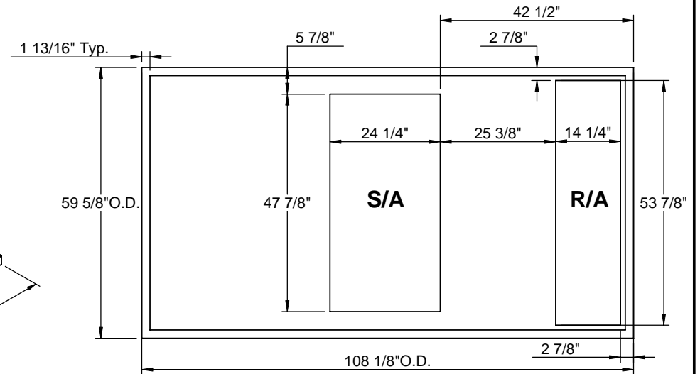
EXISTING CURB
