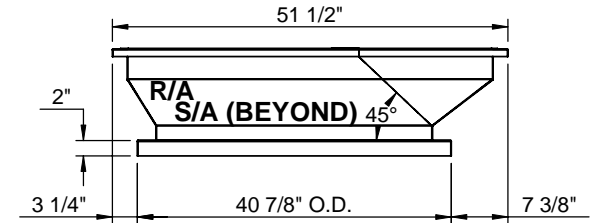
RIGHT VIEW
