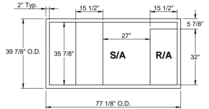
EXISTING CURB
